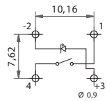
Single LED
